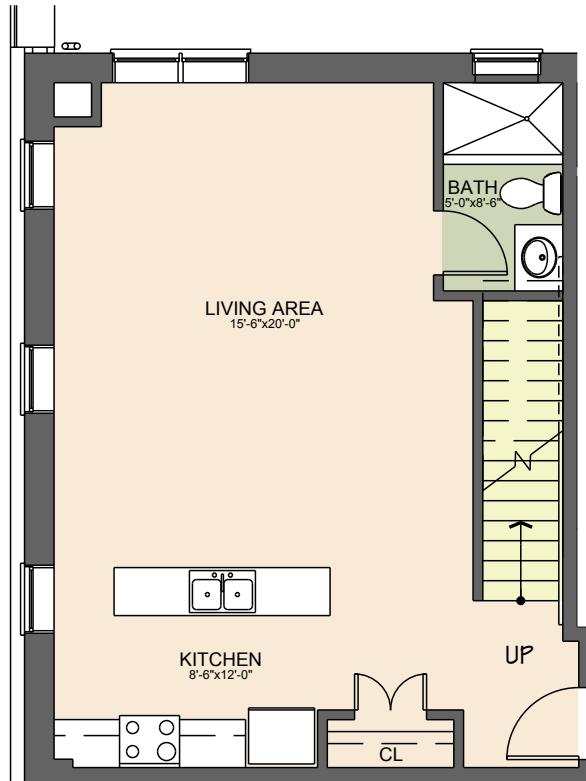
2ND FLOOR - LOWER LEVEL
