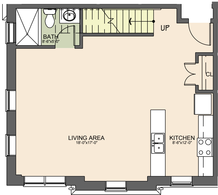
2ND FLOOR - LOWER LEVEL
